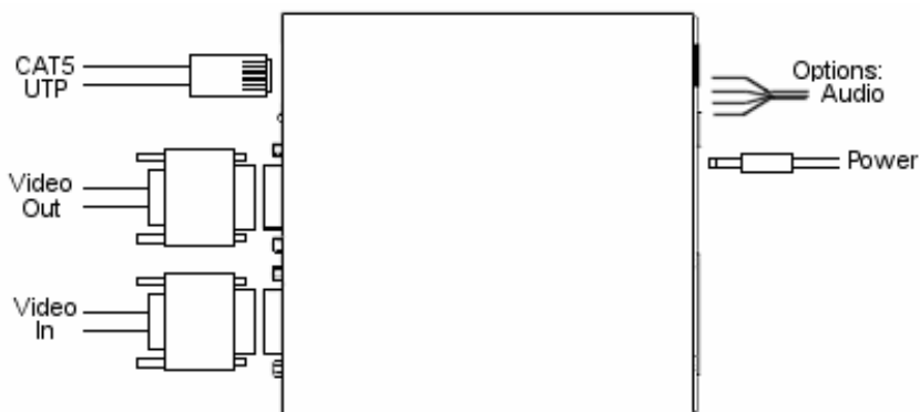
Figure 1: Transmitter Connections
